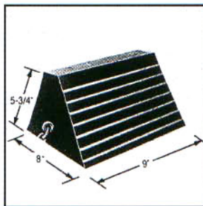
Model 68-9
