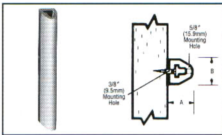
Model D-2
