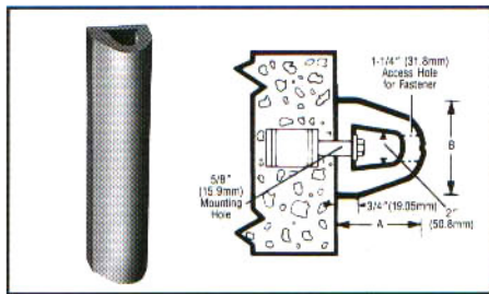
Model D-4
