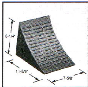
Model 811-7
