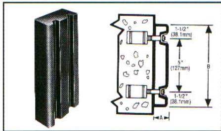
Model E
