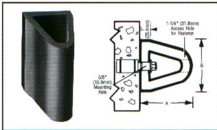
Model D-6
