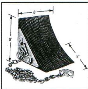
Model 88-8
